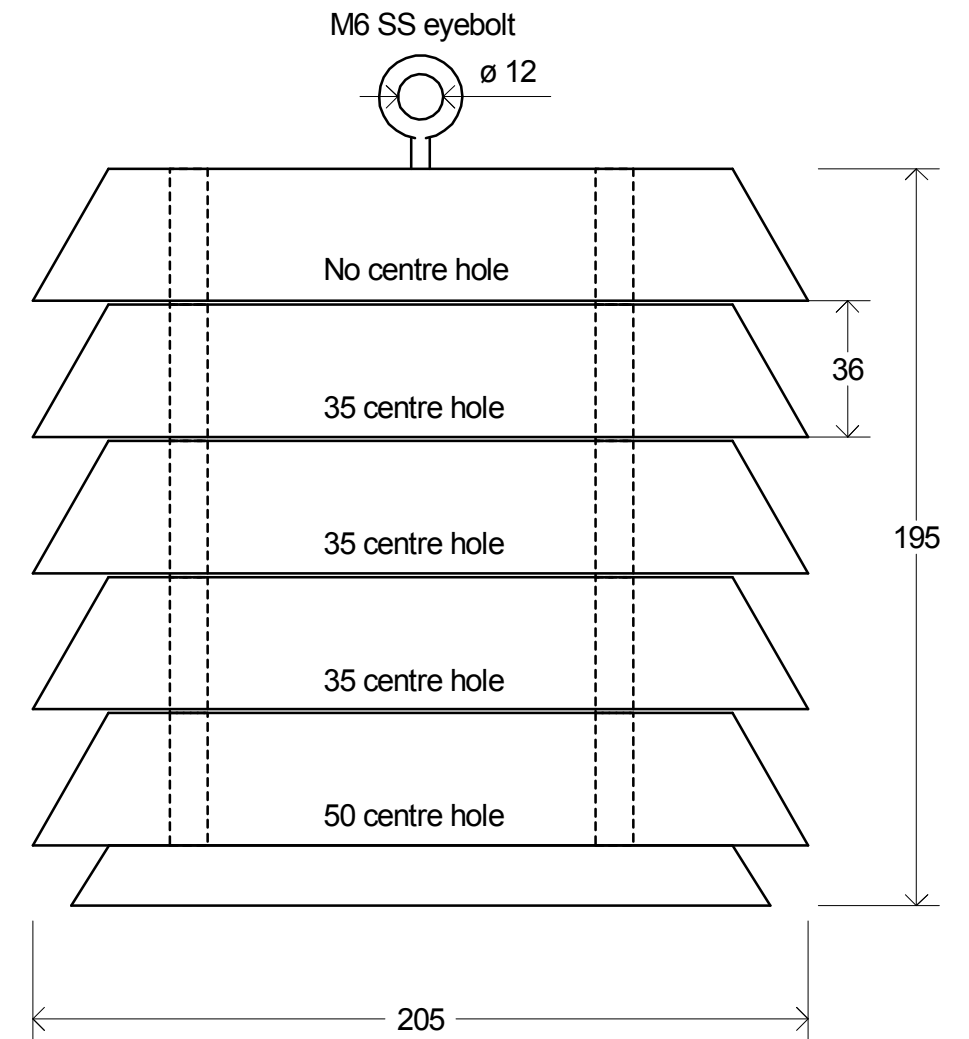
Side view
