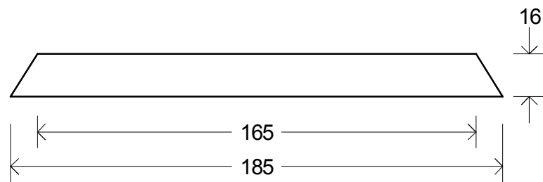
Base plate
